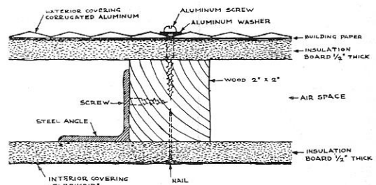
DETAILS OF WALL CONSTRUCTION
